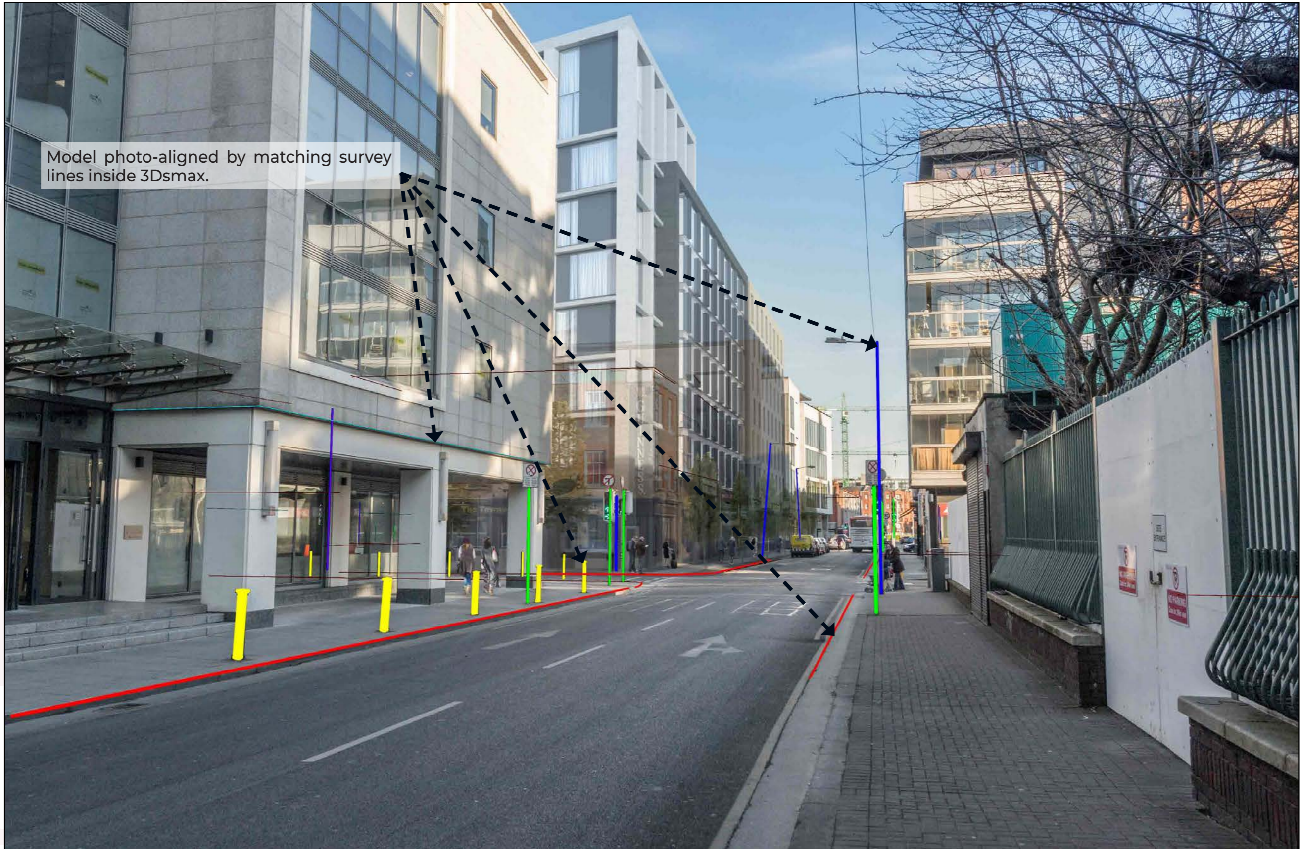
Fig.13: Fixed reference points modelled, 'rendered' and overlaid on baseline photo confirming accuracy
